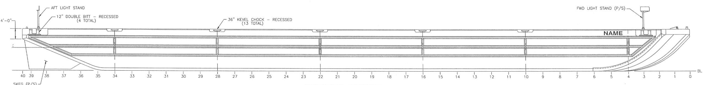
OUTBOARD PROFILE
