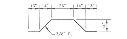
TYPICAL CORRUGATION PROFILE PROFILE TYPICAL FOR LONGITUDINAL & TRANSVERSE BULKHEADS
